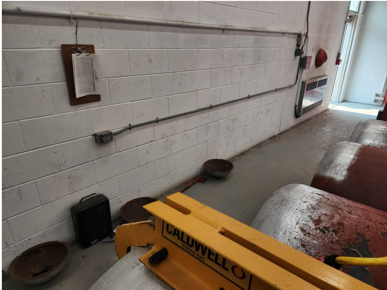
PHOTOGRAPH 10: McPhillips Regional Pumping Station – Chlorine Tonner Room Ceiling Area East Wall.
