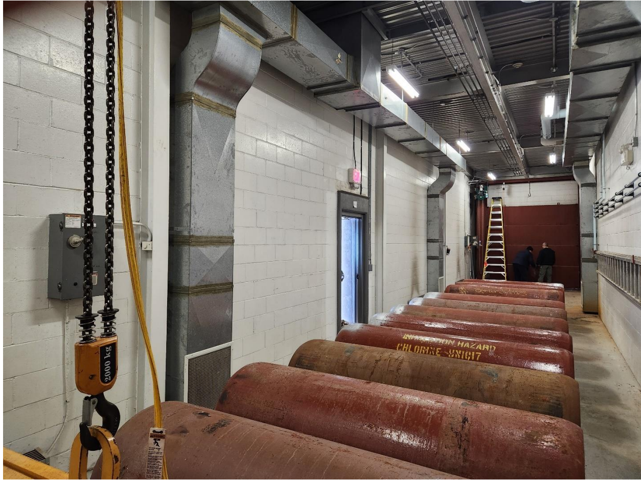
PHOTOGRAPH 52: Hurst Regional Pumping Station – Chlorine Tonner Room
