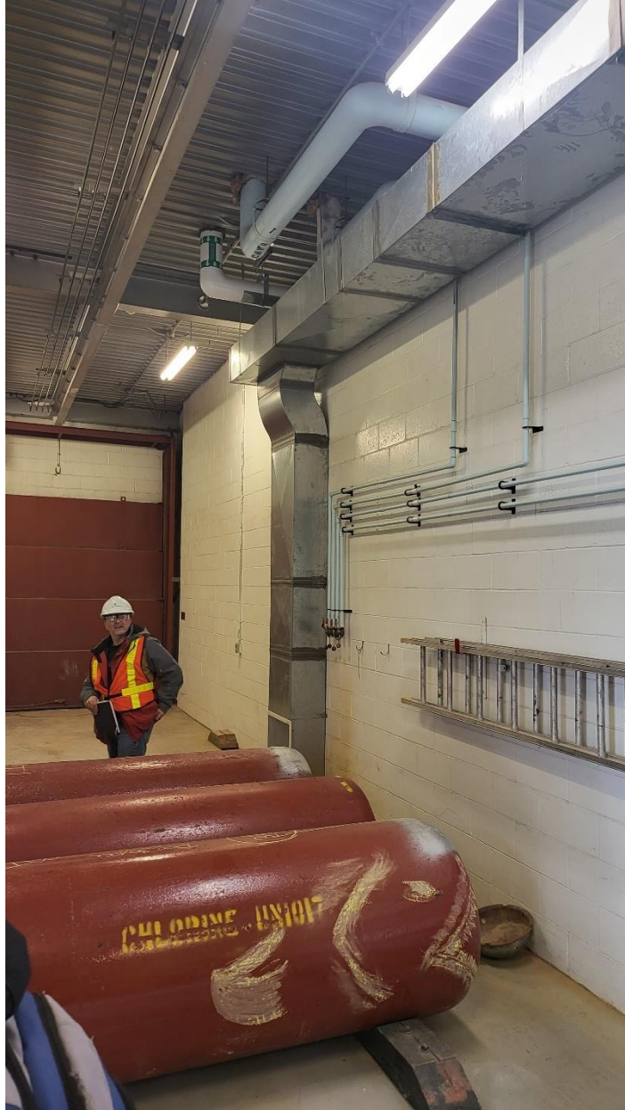
PHOTOGRAPH 53: Hurst Regional Pumping Station – Chlorine Tonner Room
