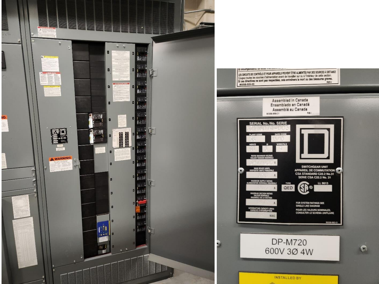
PHOTOGRAPH 38: MacLean Regional Pumping Station – Pumphouse Electrical Room - 600V Distribution DP-M720.
