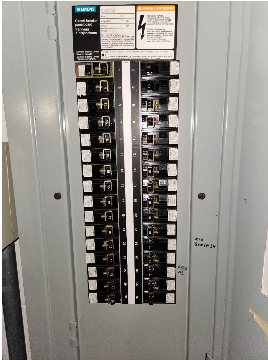
PHOTOGRAPH 63: Hurst Regional Pumping Station – Pumphouse Electrical Area – UPS Panel
