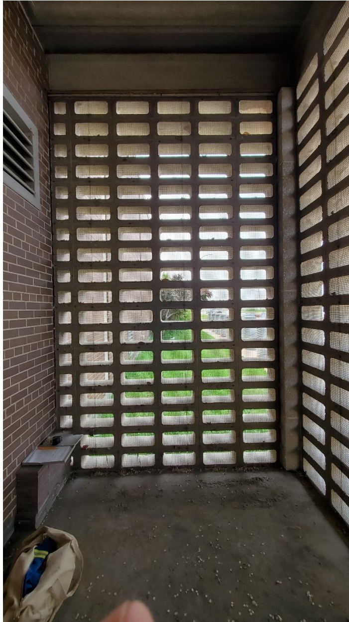
PHOTOGRAPH 33: MacLean Regional Pumping Station – West Vestibule Area to Chlorine Building.
